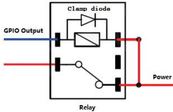
Typical relay connection
